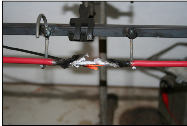
Figure 6: Cable upon completion of test
