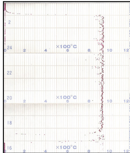
Figure 4: Strip-chart of flame temperature during test
